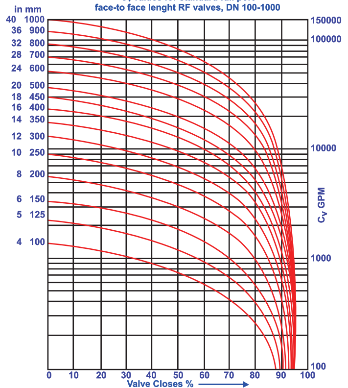
C_v values for standard full port face-to-face length RF valves, DN 100-1000
