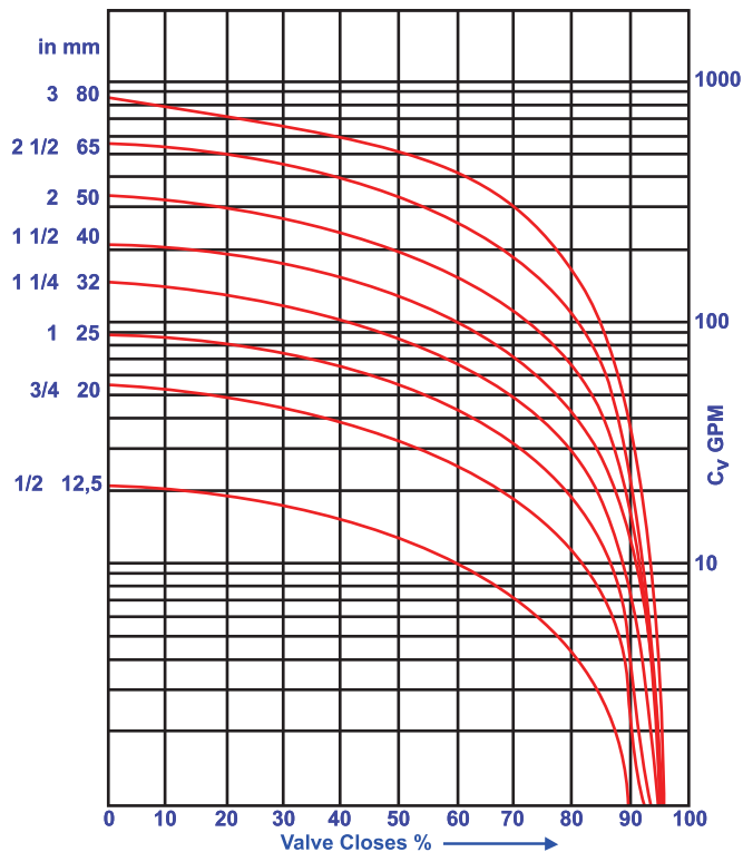
C_v values for standard full port face-to-face length RF valves, dia 25-80 mm ( C_v values for conical tubes dia 12, 15 and 18mm)
